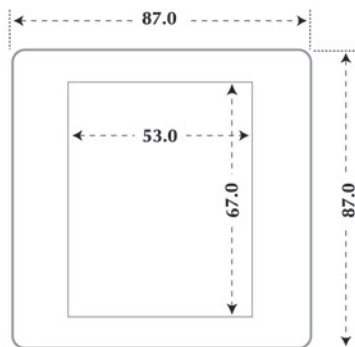
Model : A5-XXX33 Model : S13-XXX33
