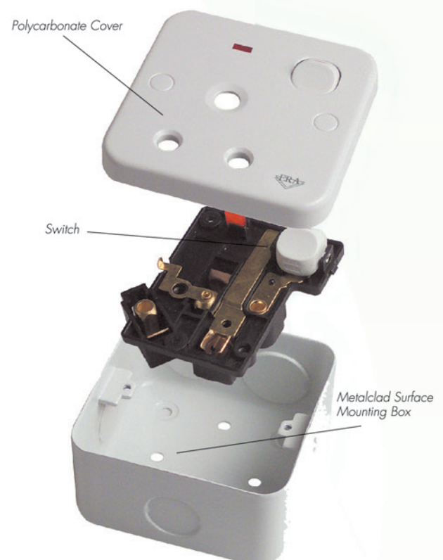
Metalclad Surface Mounted Switched Socket Outlet
