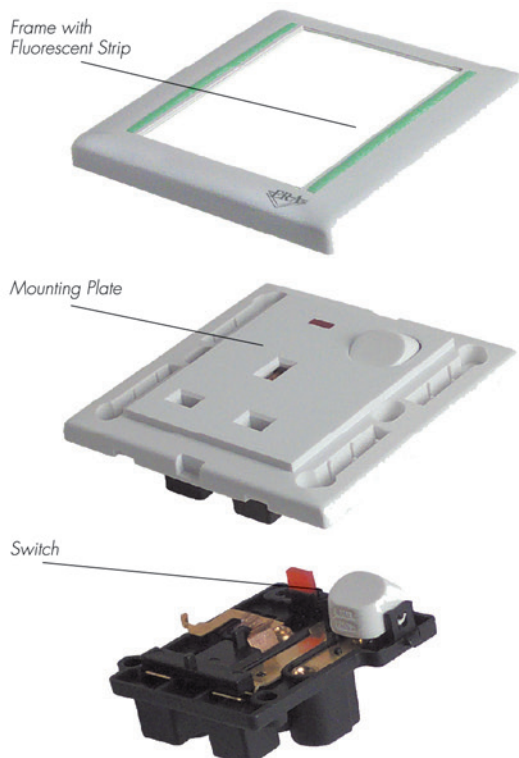
Flush Switched Socket Outlet
