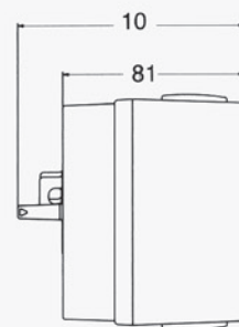
[SIDE]
